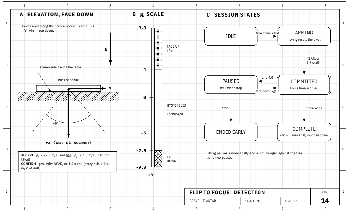
Figure 14. Flip detection. Left: the device axes and the gravity vector in the face-down position, with the accepted angular range. Centre: thresholds along the z axis, including the dead band between face-down and face-up. Right: session states; lifting the phone pauses the session and laying it down resumes it. Focus time accrues only in the COMMITTED state.
